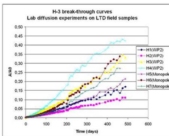
Fig. 1. Breakthrough curve range for lab through-diffusion experiments with rock samples from the LTD field experiments.
