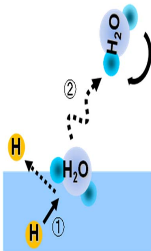
Figure 1 Schematic illustration for photodesorption of H 2 O molecule from amorphous solid water via “kick-out” mechanism by a hot H atom released from photodissociation of amorphous water ice. The numbers dedicate for sequence of the reaction.
