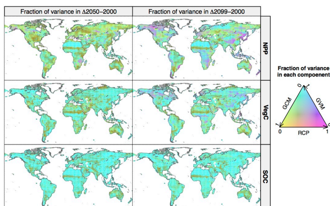
Figure 1. Relative importance of each uncertainty source to \Delta NPP, \Delta VegC, and \Delta SOC (from Nishina et al., 2014 in ESDD)
