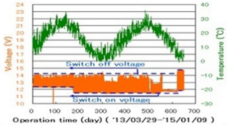
Fig.2 Long Term DMFC Operation Test
