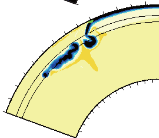
with back-arc spreading and hot material
