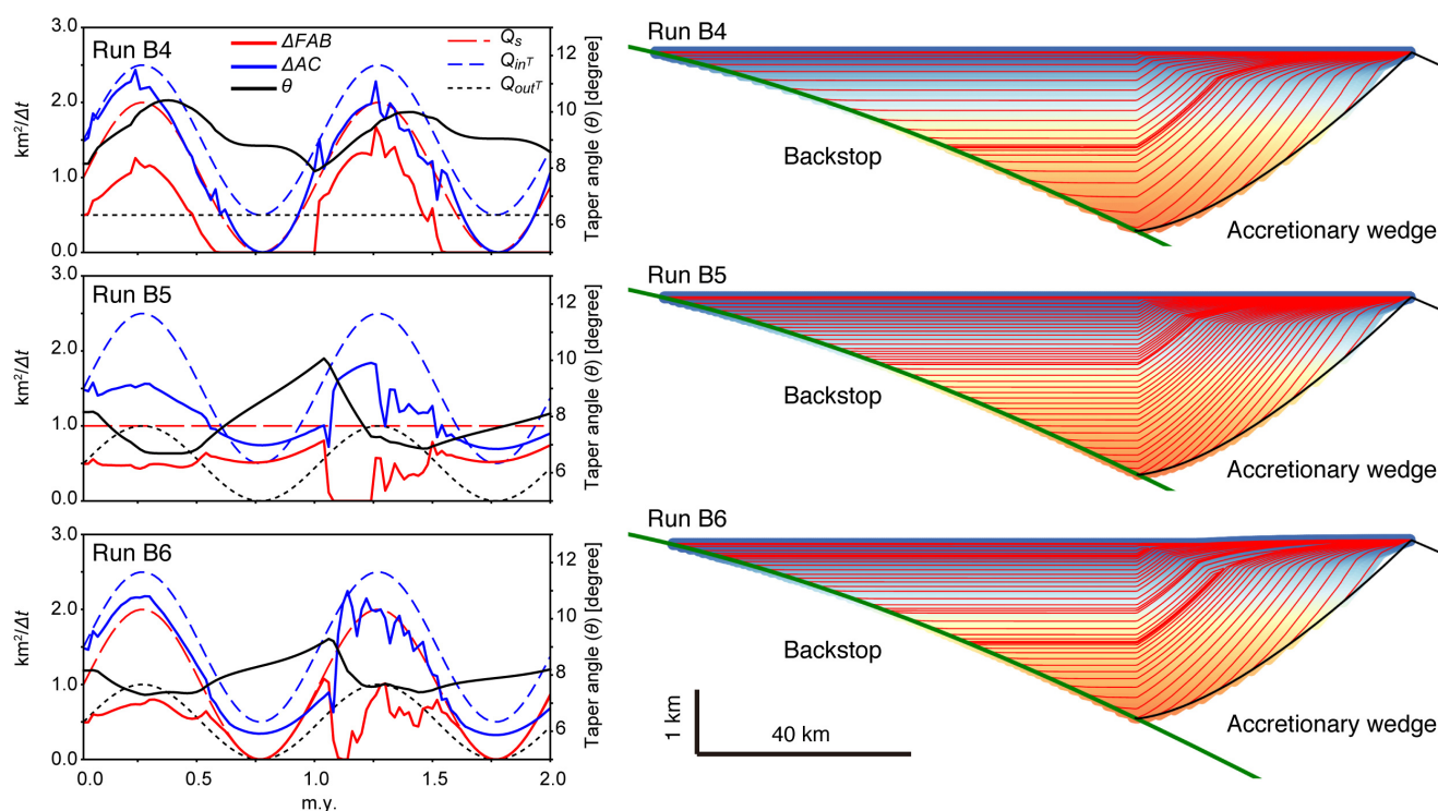
Fig. 1: Selective examples from the dynamic taper models. (Left) Diagrams for initial parameters of Q_s , Q_{inT} , and Q_{outT} (see the text for notations), taper angles ( \theta ), and increased areas of forearc basin ( \Delta FAB ) and accretionary wedge ( \Delta AC ) at each time step. (Right) Resultant stratigraphy of forearc basins.
