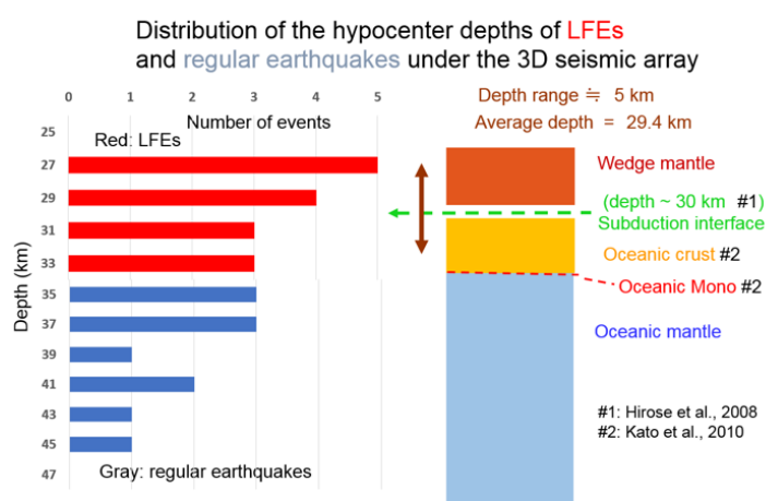
Fig.2. Comparison of hypocenter depth distributions (left) with schematic inter-plate structure (right).
