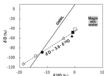
Fig. 2. \delta\text{D} vs. \delta^{18}\text{O} diagram of condensed water of samples.
